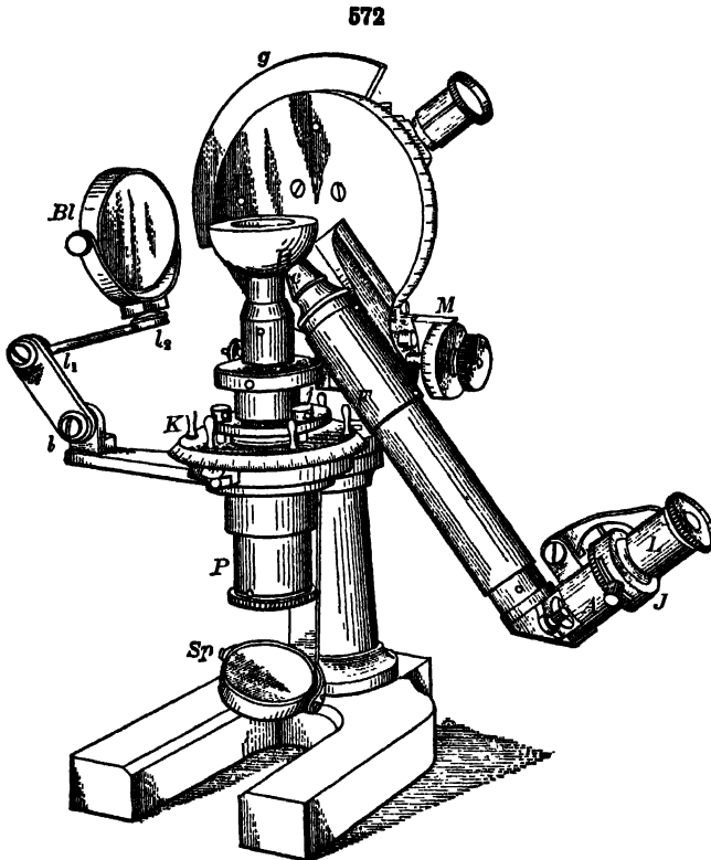
Total Refractometer
